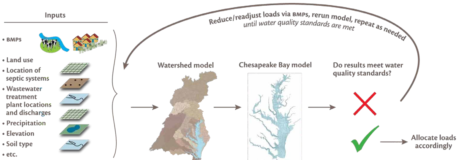
Figure 3. Simplified schematic of how pollution reduction goals were determined for the Chesapeake Bay TMDL using environmental models. The models used are complex mathematical representations of the real world, based on up-to-date peer-reviewed science, that produce estimates of how pollutant loads to the Bay change under different management scenarios (i.e., implementation of different kinds of BMPs).
